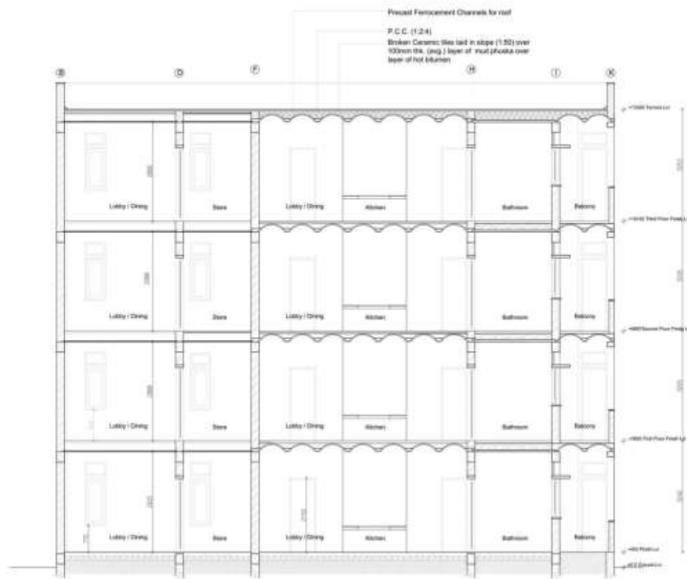
SECTION Y-Y'
