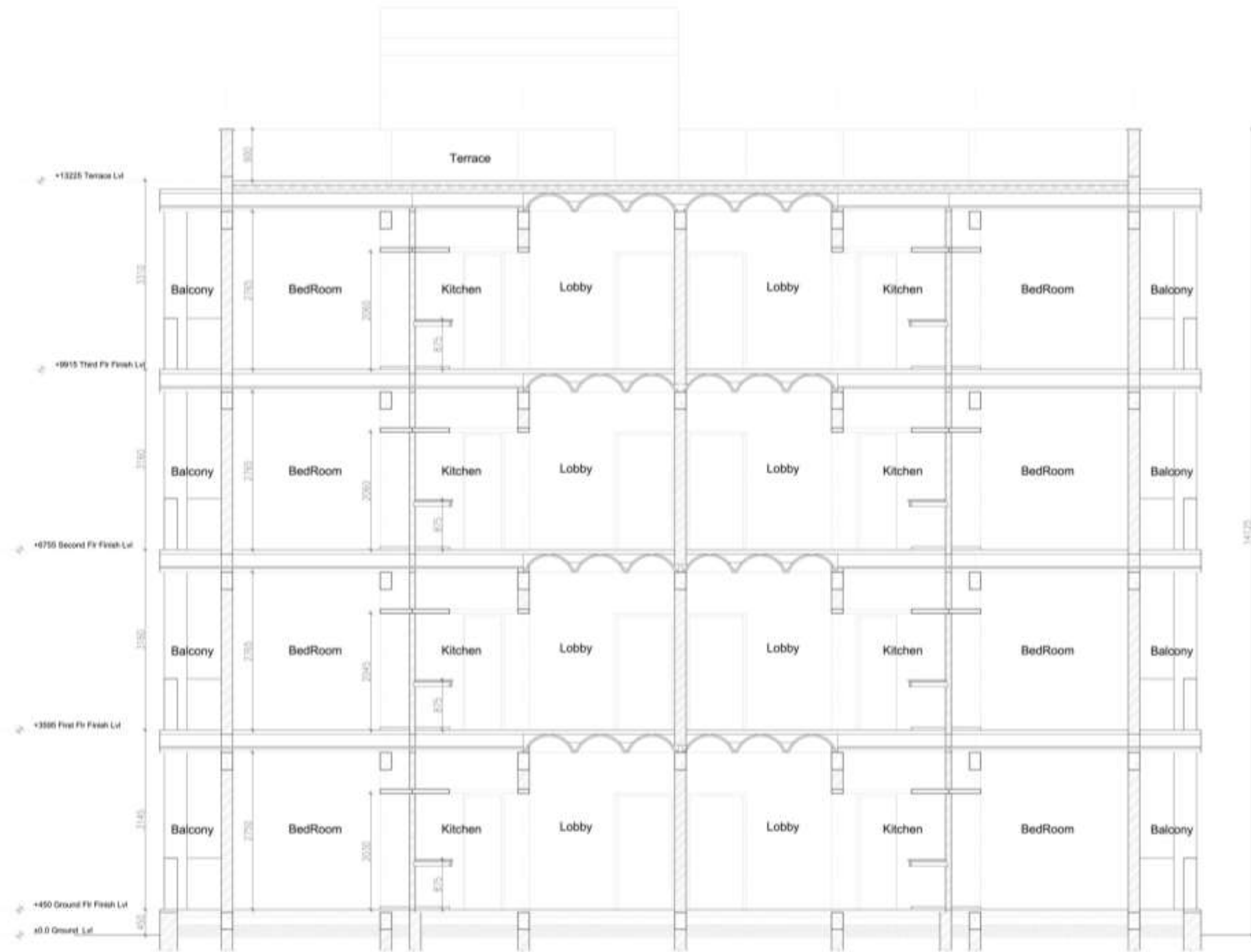
SECTION Y-Y
