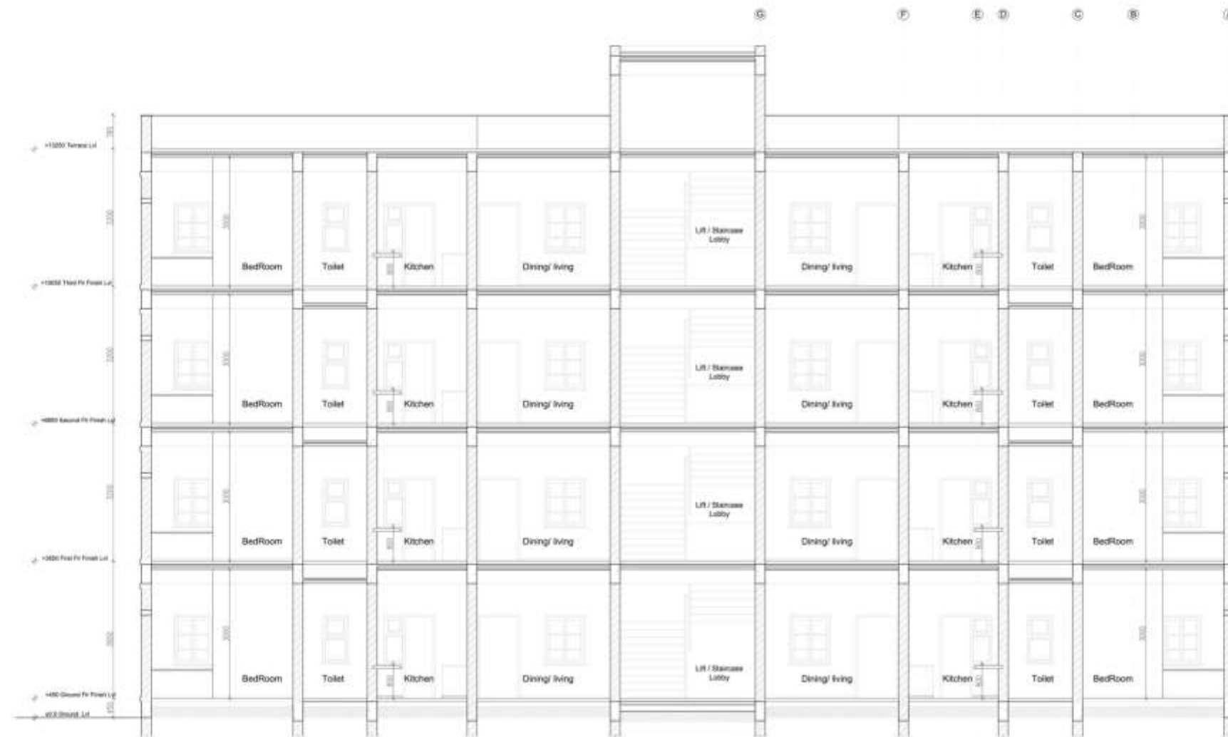
SECTION Y-Y
