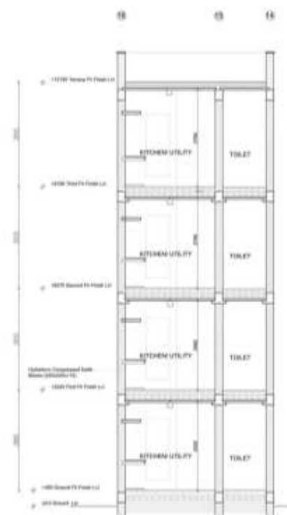
SECTION Y-Y'
