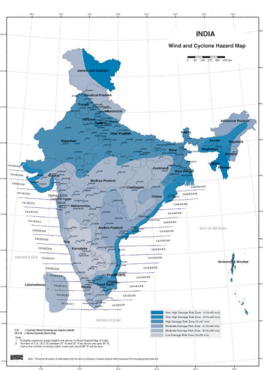
Figure 4: Wind and Cyclone Hazard Map of India
