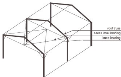
(b) Eaves level knee bracing
