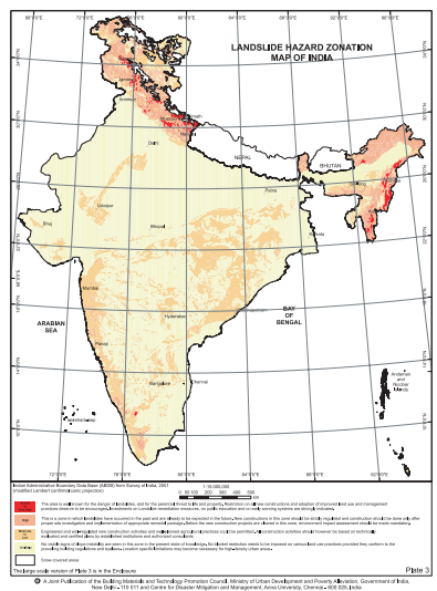
Figure 5: Landslide Hazard Map of India
