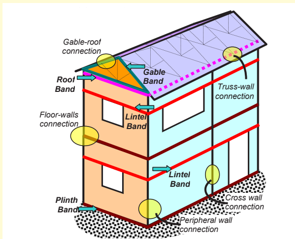
Figure 7: Horizontal bands in masonry building
