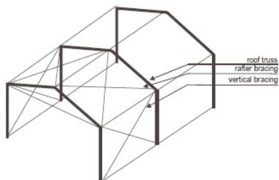
(a) Bracing in rafter plane
