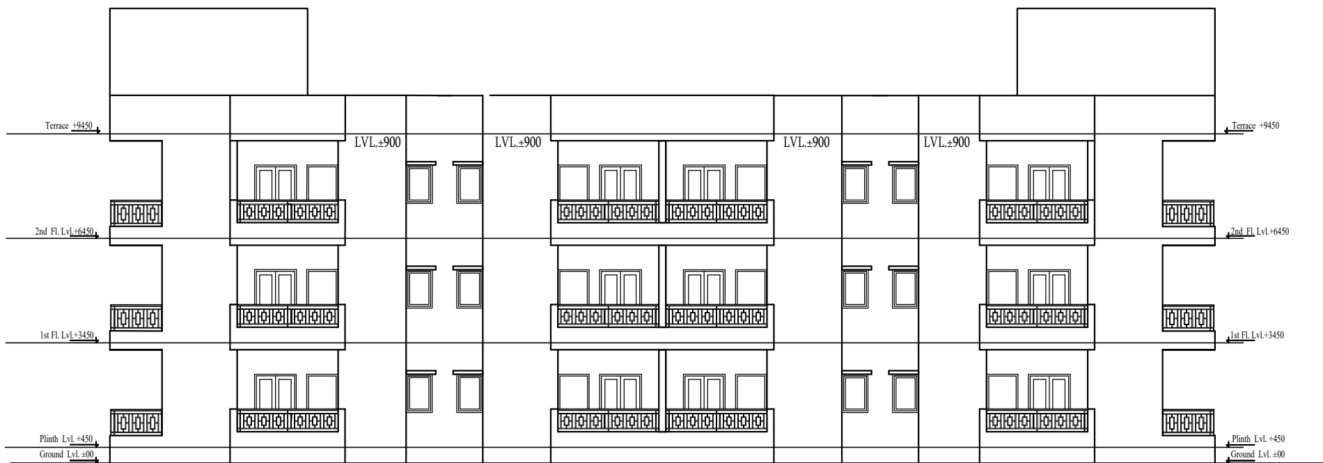
REAR ELEVATION -B
